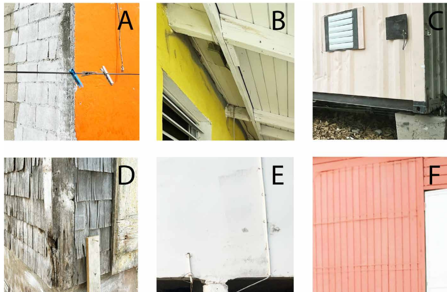
FIG. 2.7 Building materials used for structure: (A) concrete blocks; (B) concrete wall and timber rafters; (C) container on poured concrete pillar. Materials used for skin: (D) wooden shingles; (E) cement; (F) wooden cladding.
