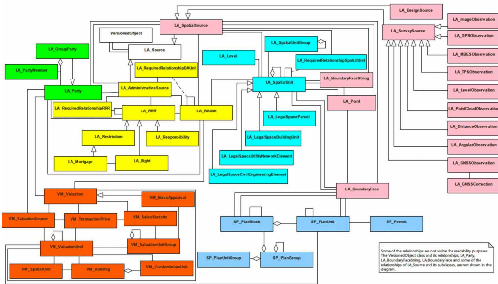
FIG. 4.10 Parts 1, 2, 4 and 5 of LADM Edition II and their relationships (Kara et al., 2024a)
