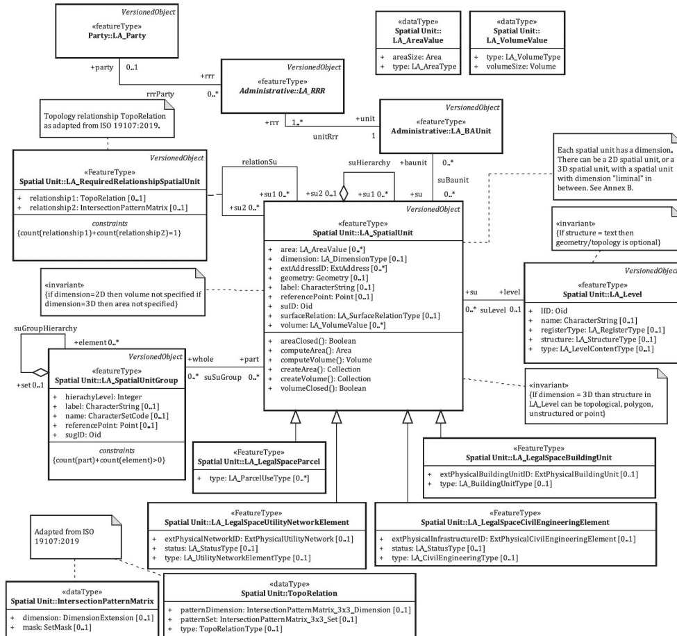
FIG. 6.9 Subclasses of LA_SpatialUnit of the Spatial Unit Package of the LADM survey model, with associations to other basic classes
