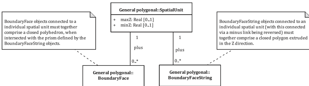
FIG. 6.5 Conceptual model of the “general spatial unit in polygonal encoding” (simplified) spatial profile
